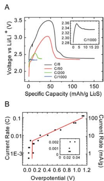
Figure 5. Relation between current rates and overpotentials. (A) Initial potential barrier at C/8, C/50, C/200, and C/1000. 1C = 1166 mA/g. (Inset) Zoom-in image of the barrier at C/1000. (B) Relation between the current rate and the overpotential. There are two regions. At rates higher than C/200, the overpotential depends linearly on the logarithm of the current. At rates lower than C/300, the overpotential is approximately constant. (Inset) Low rate region ( <C/300 ). Red line is for eye guiding. Units in both insets are the same as the figures.
