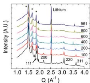
Figure 4. In-situ X-ray diffraction patterns of \text{Li}_2\text{S} electrode during the initial charging. \text{Li}_2\text{S} peaks were indicated with the indexing and disappeared on charging, but no extra peaks belonging to sulfur were detected. Numbers on the right represent the charging capacity. Asterisks (*) correspond to peaks from the plastic bag and the polymer separator.
